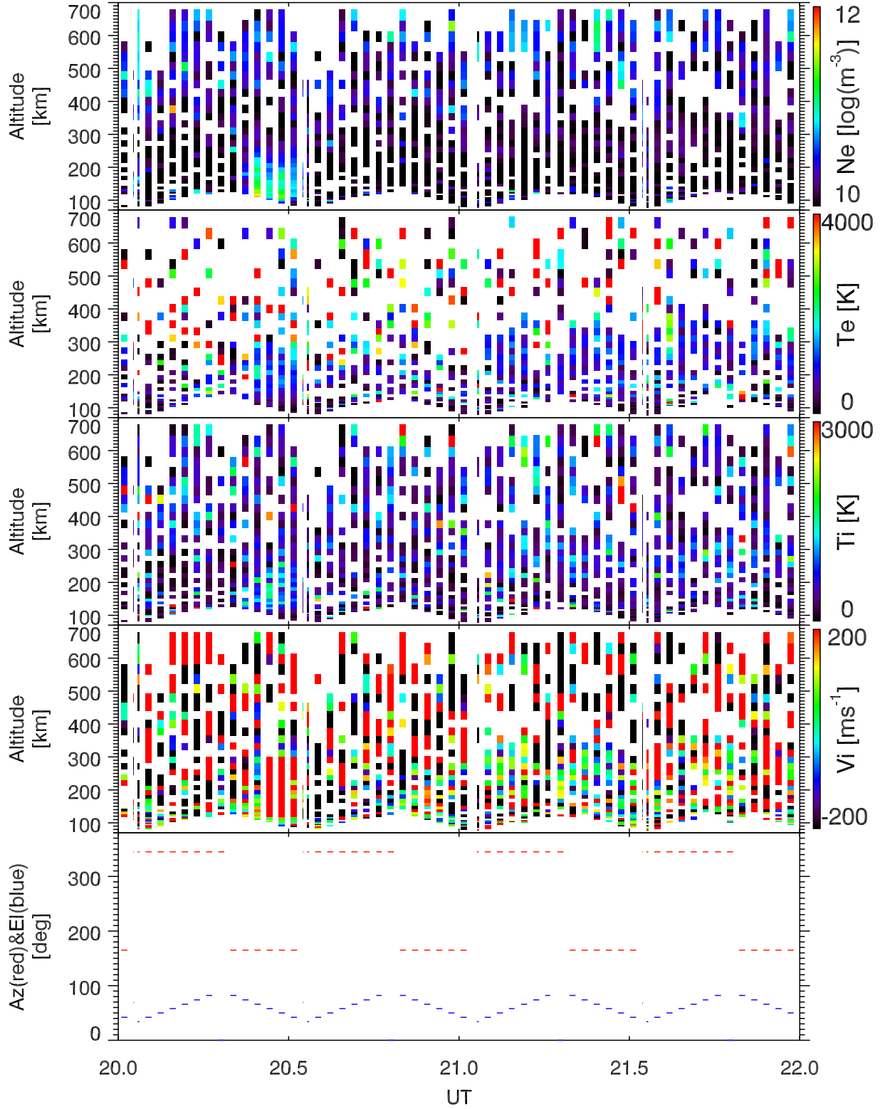
EISCAT 2006-12-17_20_22UT_tau0_ant@32m.
