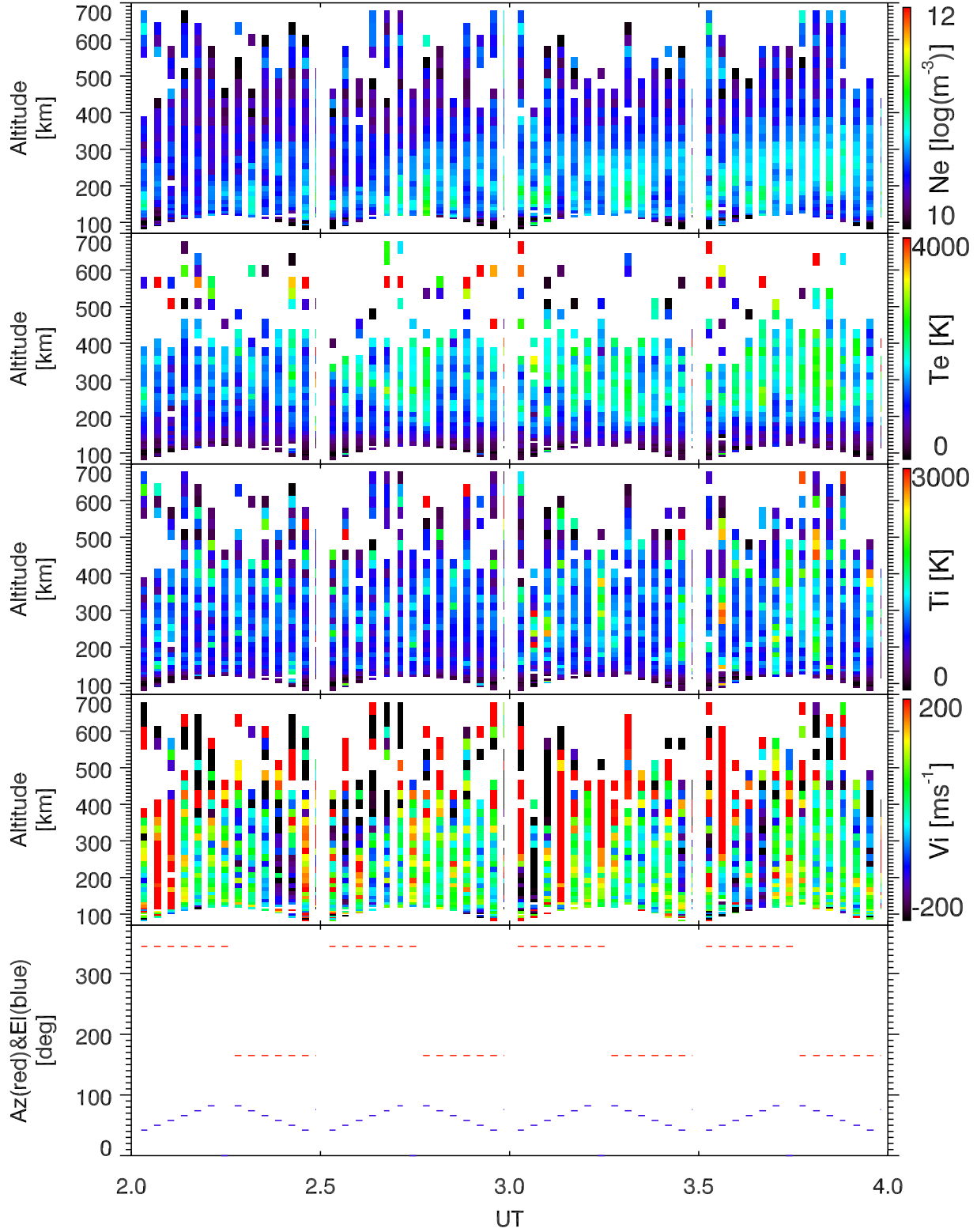
EISCAT 2006-12-19_02_04UT_tau0_ant@32m.
