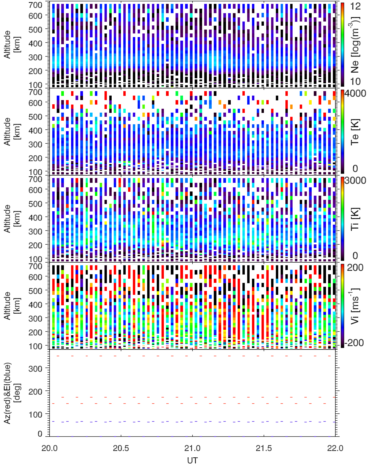
EISCAT 2007-03-01_20_22UT_steffe_ant@32m.
