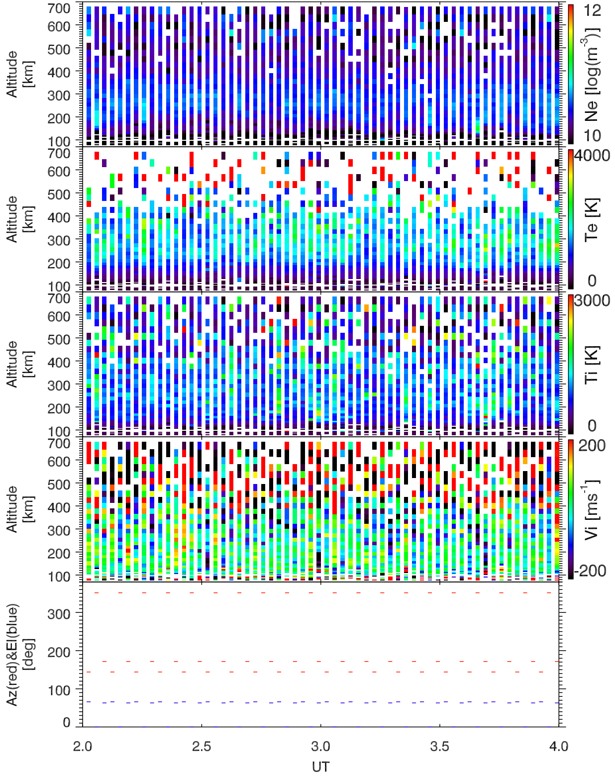
EISCAT 2007-03-02_02_04UT_steffe_ant@32m.
