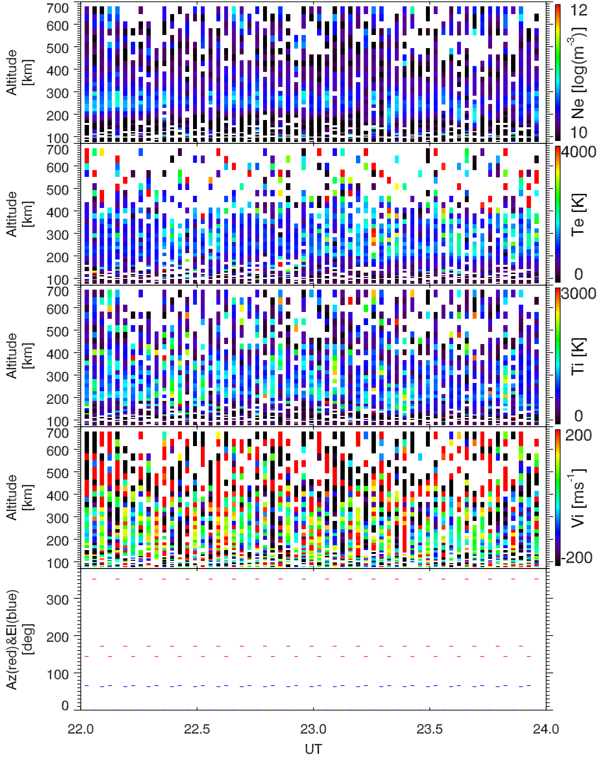
EISCAT 2007-03-03_22_24UT_all_all@32m.
