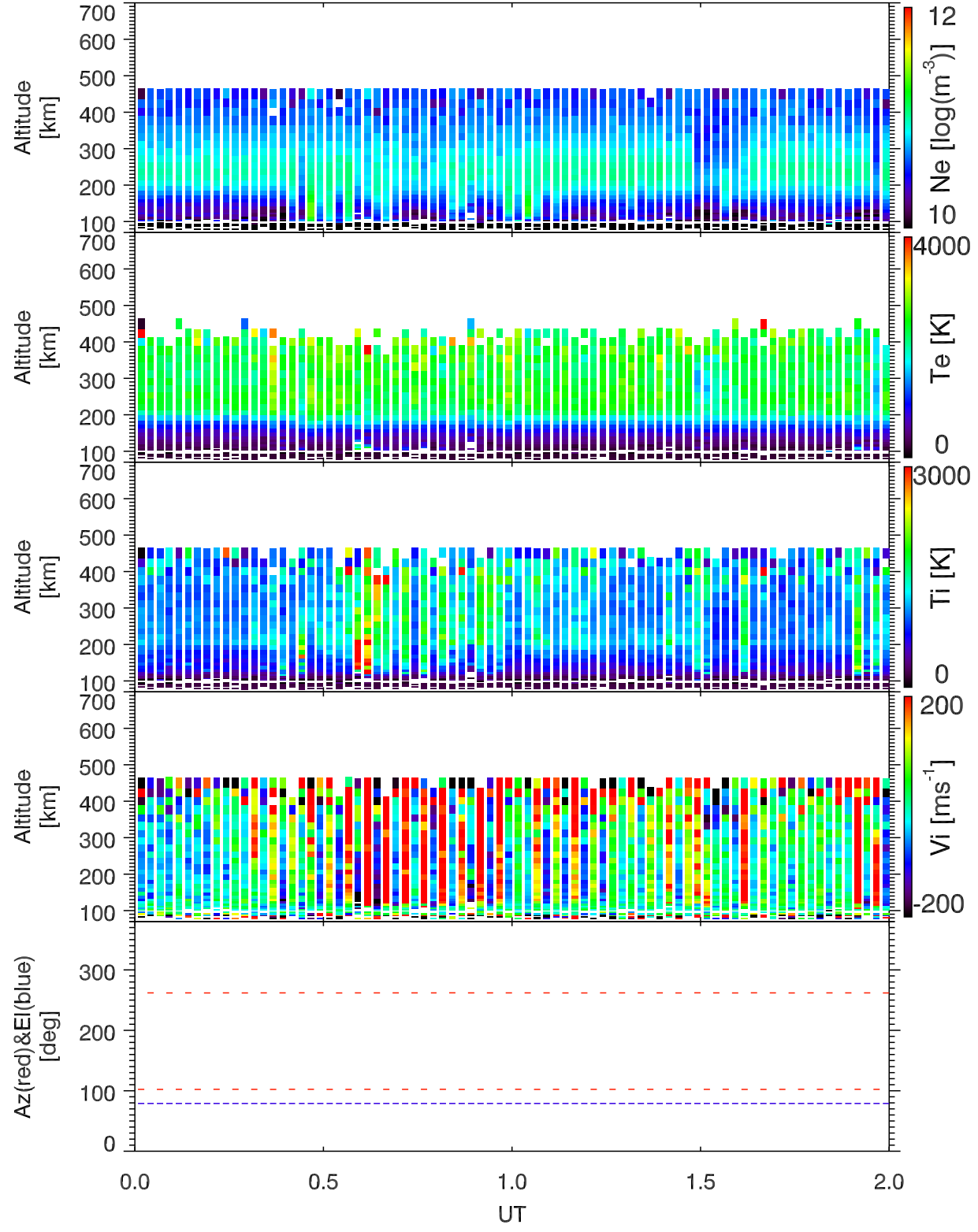
EISCAT 2007-04-27_00_02UT_ipy_ant@32m.
