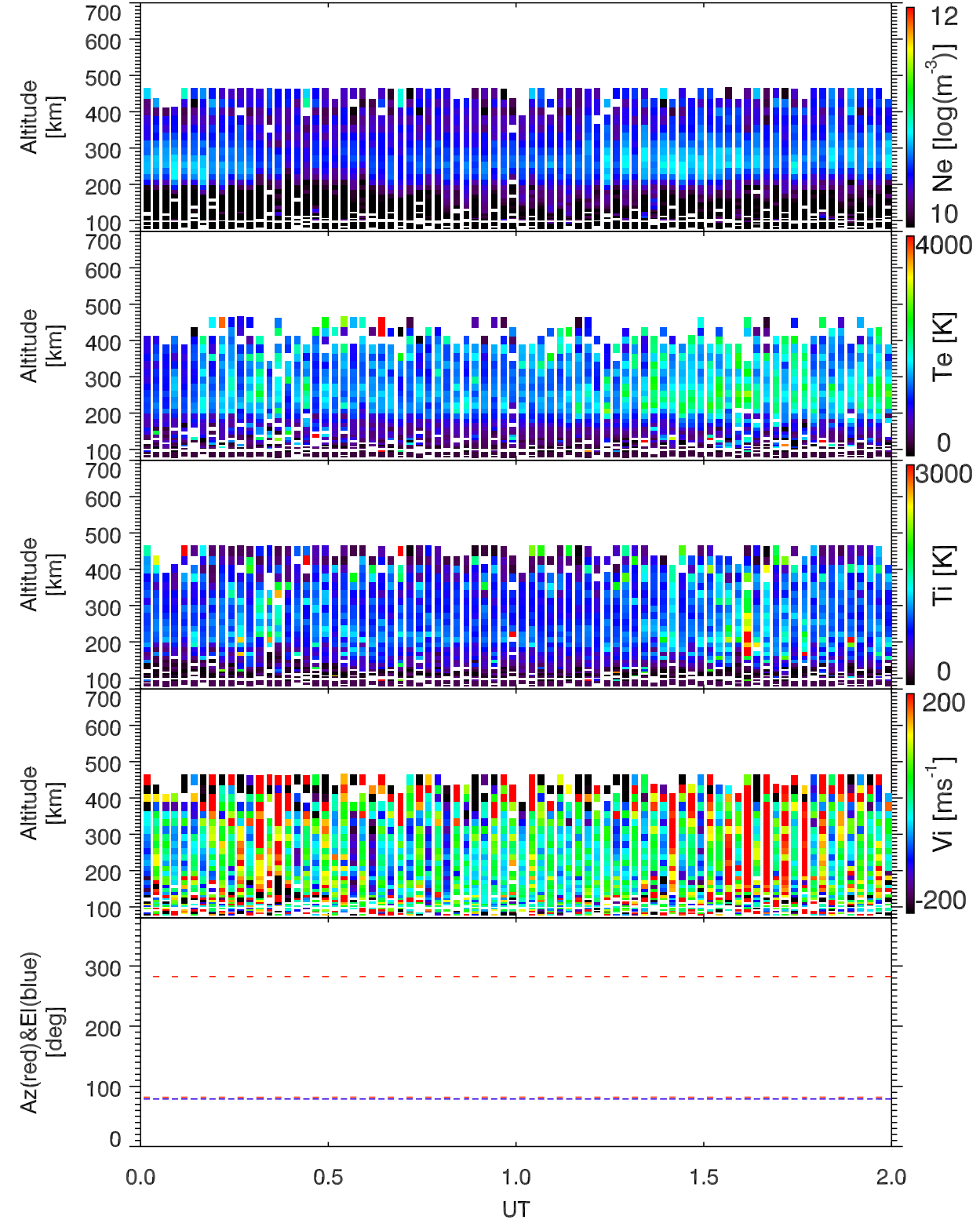
EISCAT 2007-10-12_00_02UT_ipy_ant@32m.
