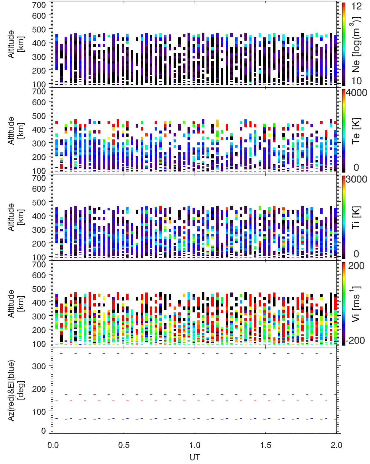
EISCAT 2007-12-14_00_02UT_ipy_ant@32m.
