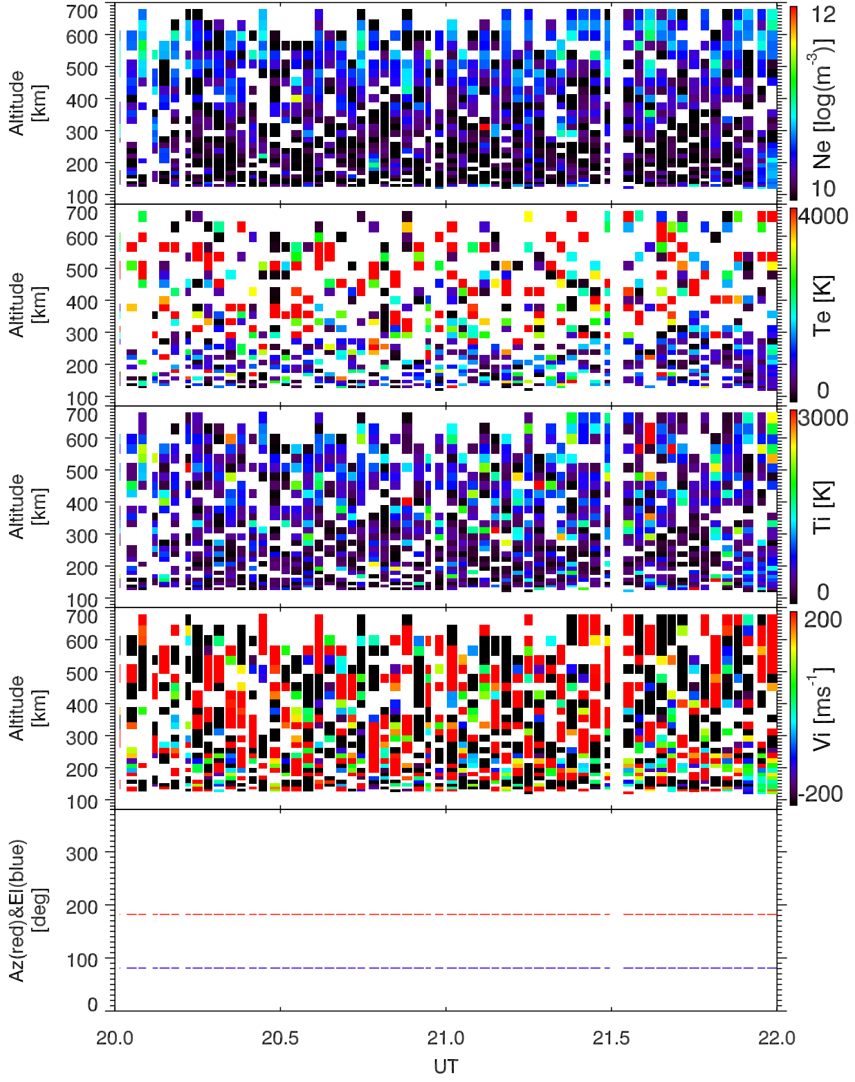
EISCAT 2008-01-30_20_22UT_all_all@42m.
