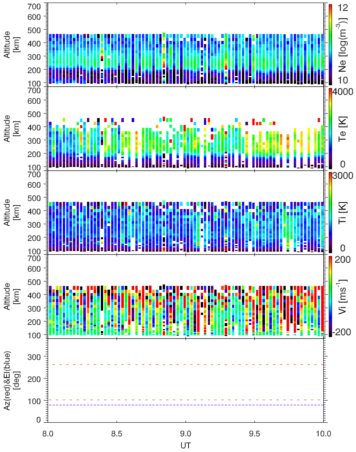
EISCAT 2008-02-15_08_10UT_ipy_ant@32m.
