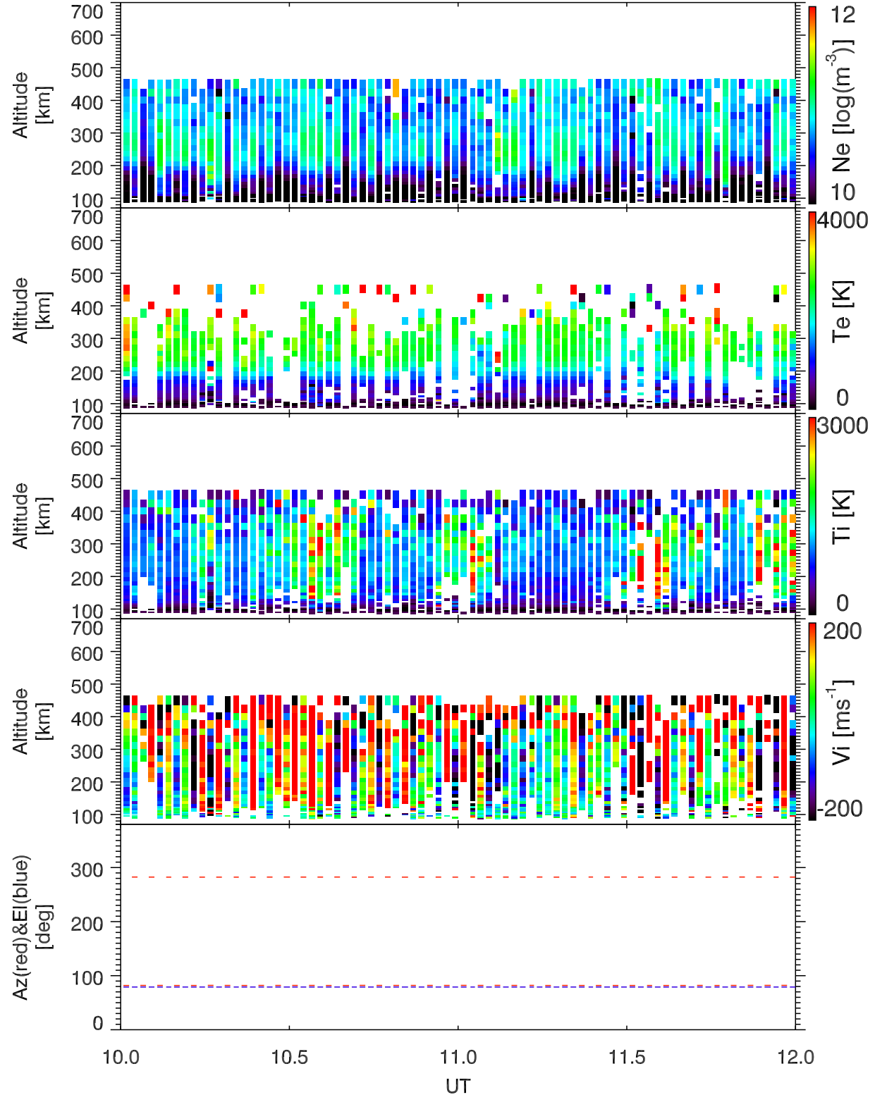
EISCAT 2008-02-29_10_12UT_ipy_ant@32m.
