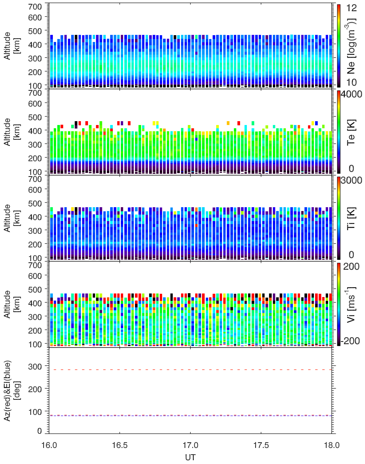
EISCAT 2008-05-09_16_18UT_ipy_ant@32m.
