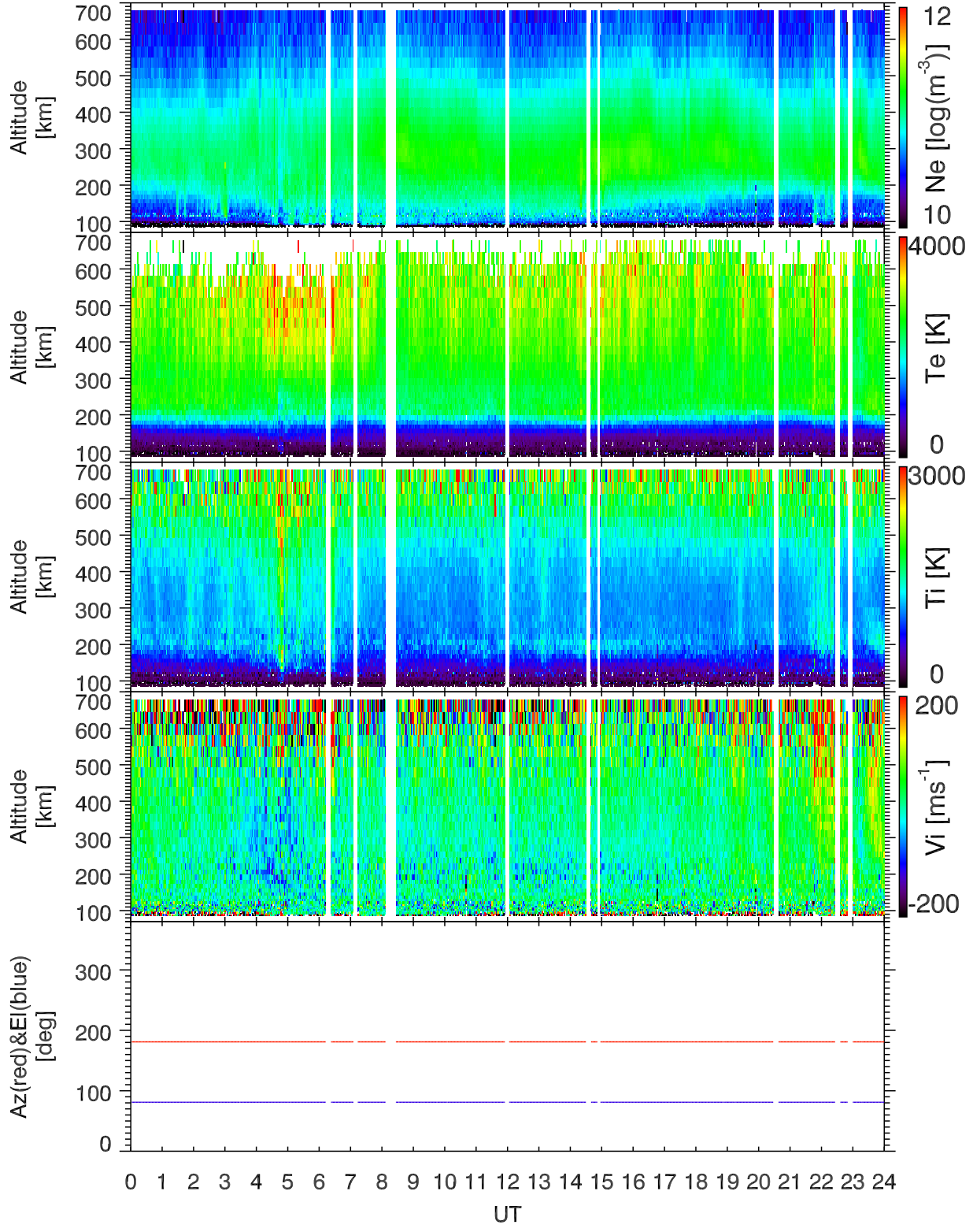
EISCAT 2004-06-03_00_24UT_tau0_120@42m.
