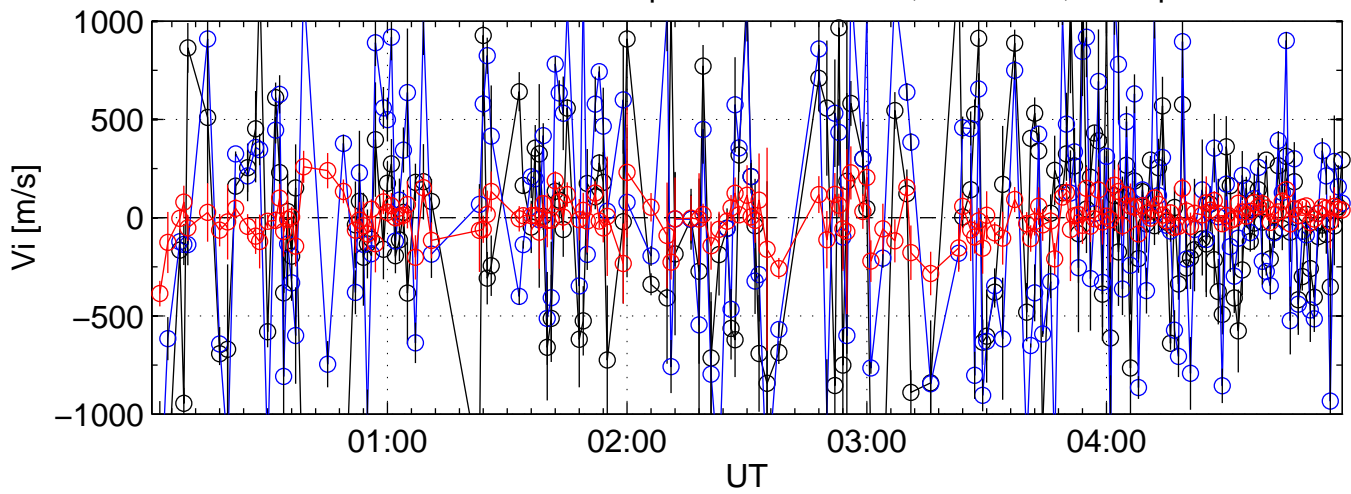
KST 2006-09-23 tau2pl@kir black:North, blue:East
