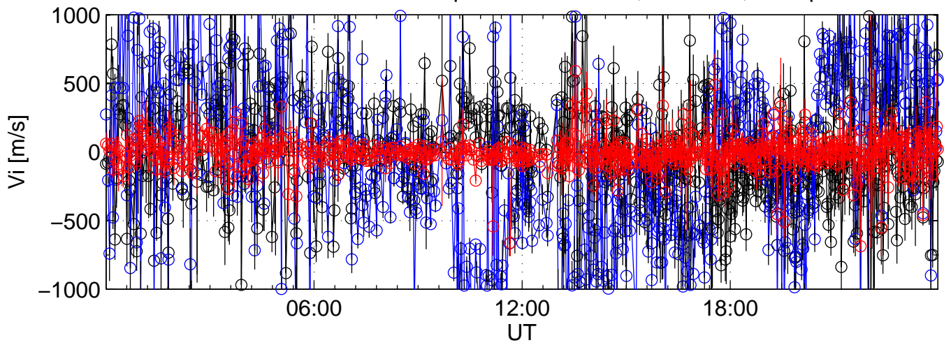
KST 2003-11-17 tau2pl@kir black:North, blue:East
