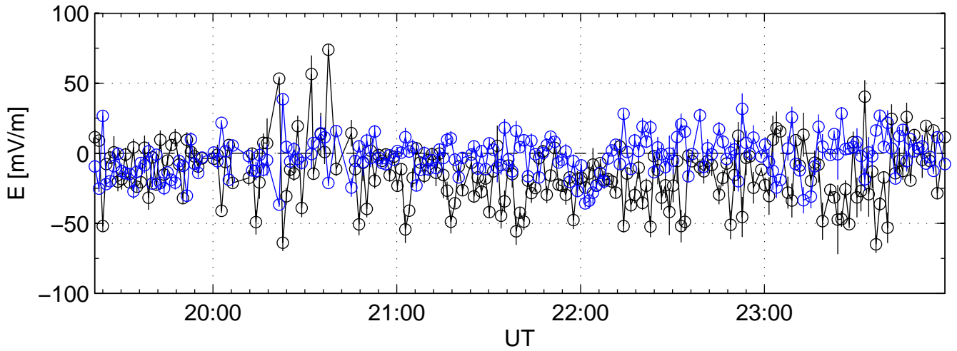
KST 2005-10-08 tau2pl@kir black:North, blue:East
