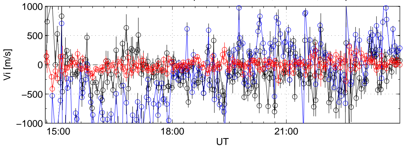
KST 2006-02-20 tau2pl@kir black:North, blue:East
