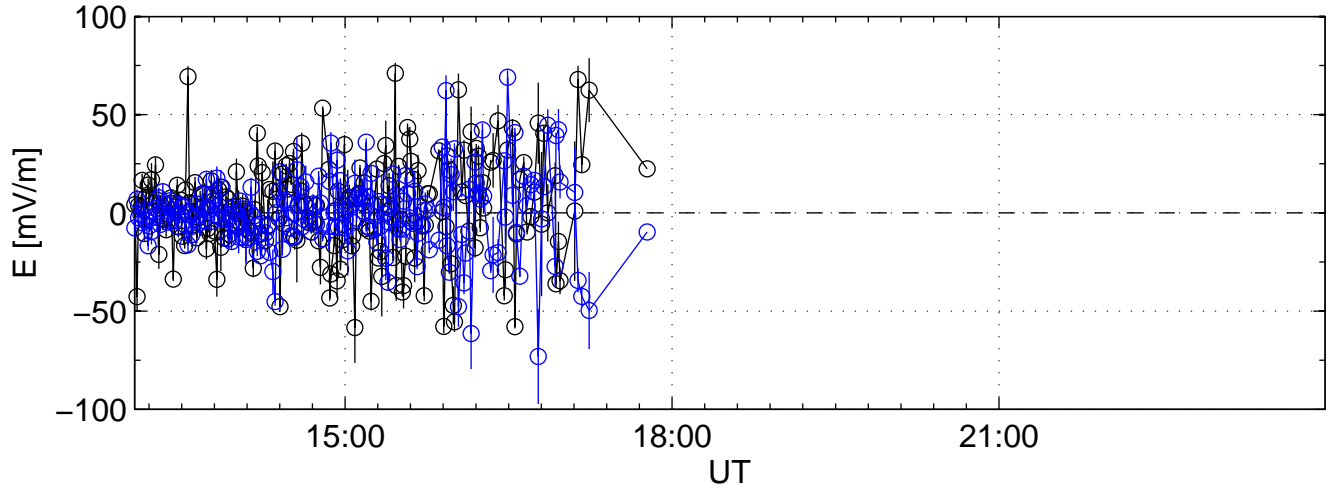
KST 2009-01-22 beata@kir black:North, blue:East
