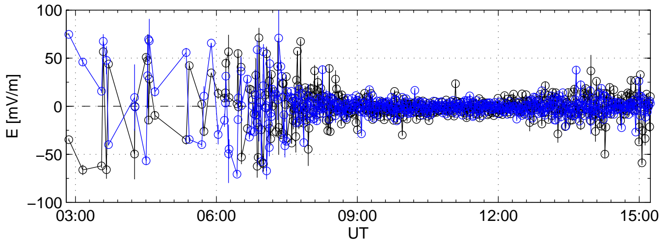
KST 2010-01-19 beata@kir black:North, blue:East
