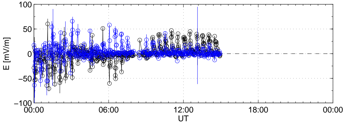
1991-03-20 kst cp3f 0000sec black:North, blue:East
