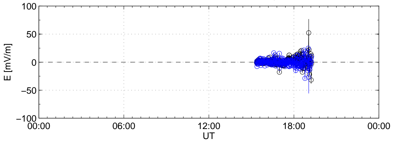
2001-11-11 kst tau2 0060sec black:North, blue:East
