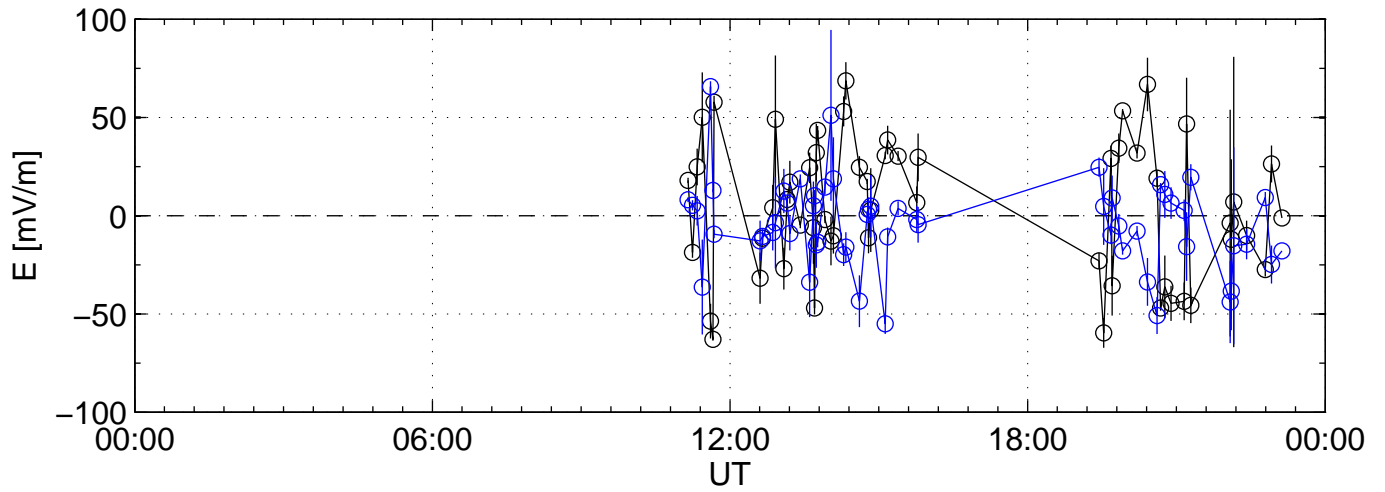
2004-05-17 kst tau1 0000sec black:North, blue:East
