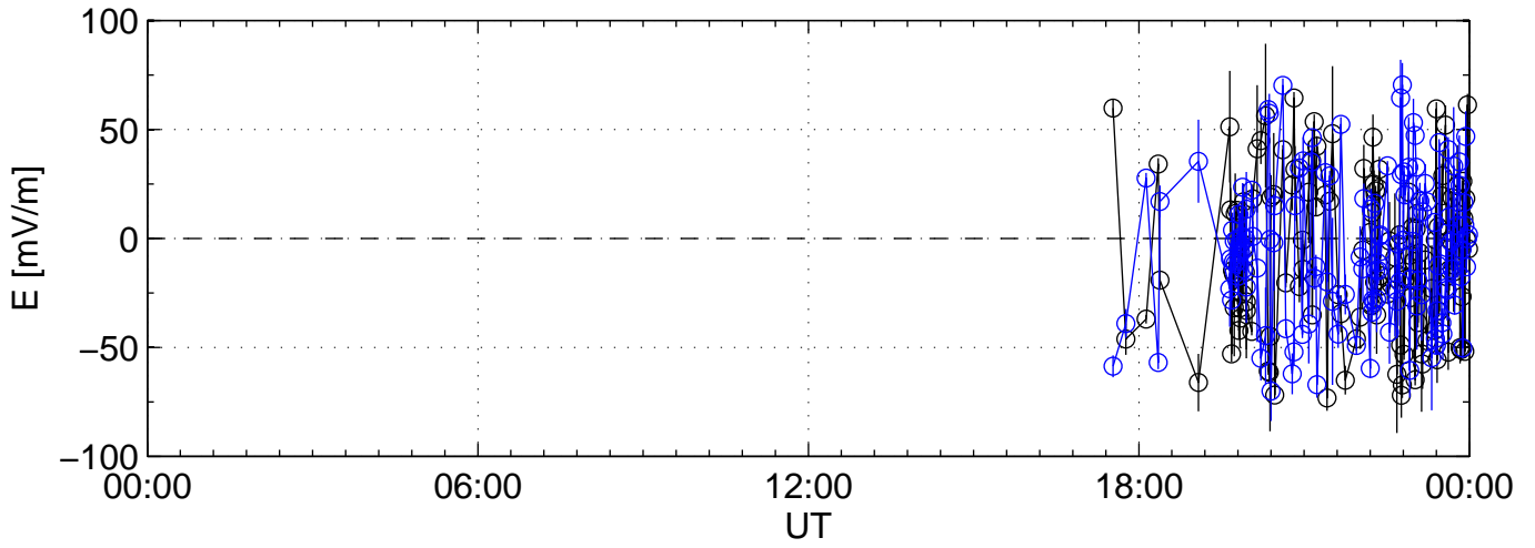
2006-10-16 kst arc1 0060sec black:North, blue:East
