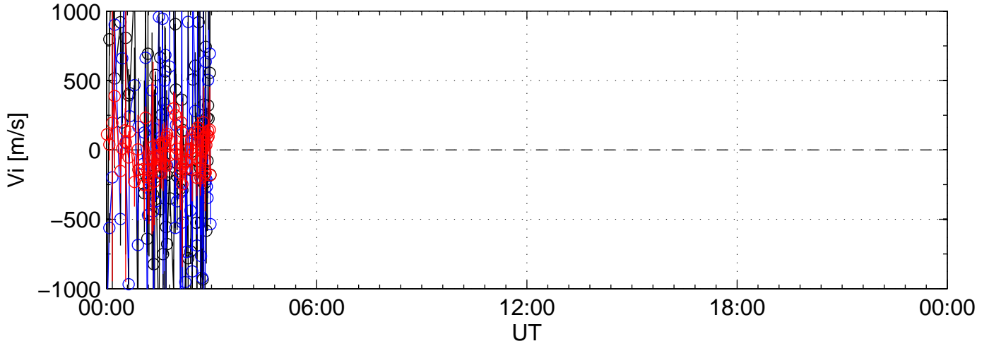
2006-11-19 kst arc1 0060sec black:North, blue:East
