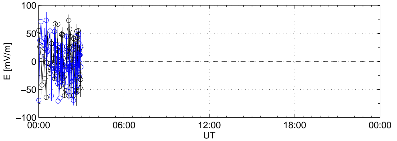
2006-11-19 kst arc1 0060sec black:North, blue:East
