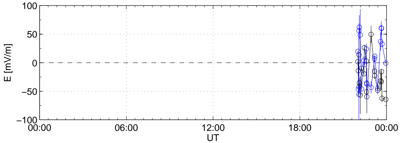
2007-11-29 kst arc1 0060sec black:North, blue:East
