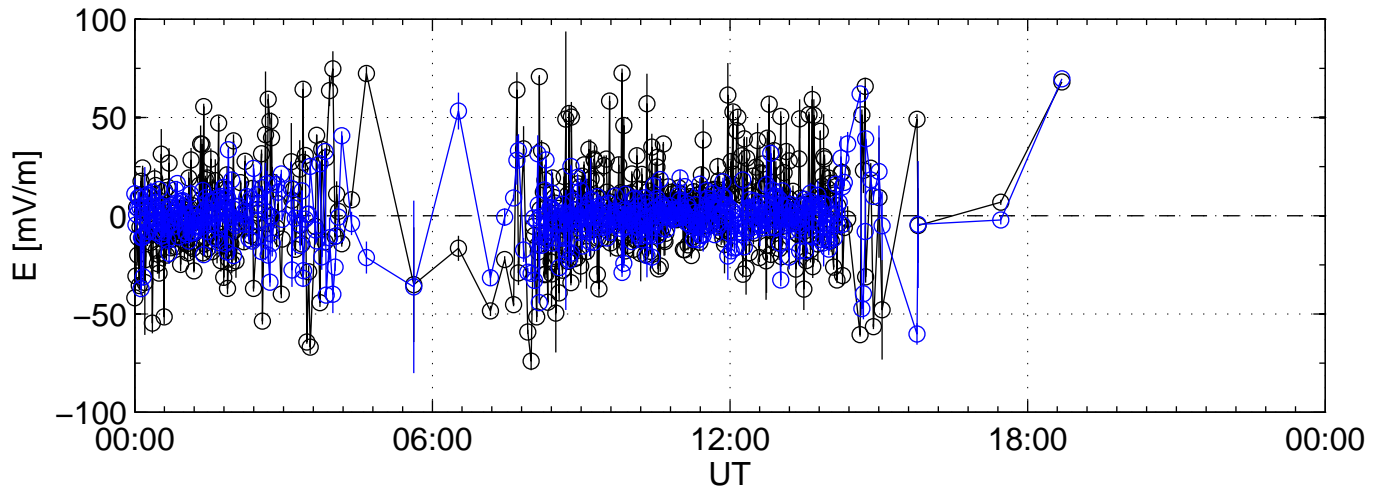
2009-01-09 kst beat 0000sec black:North, blue:East
