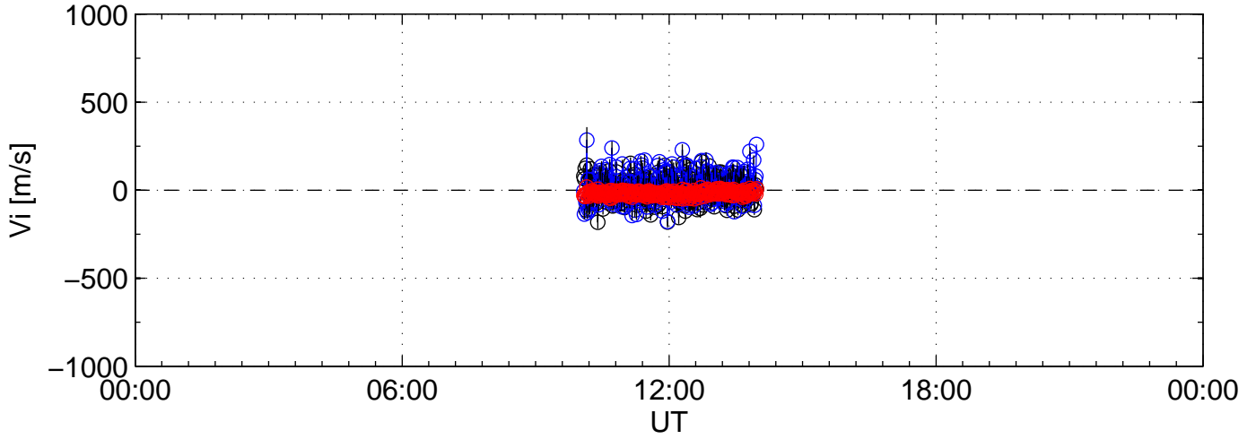
2009-09-17 kst beat 0060sec black:North, blue:East
