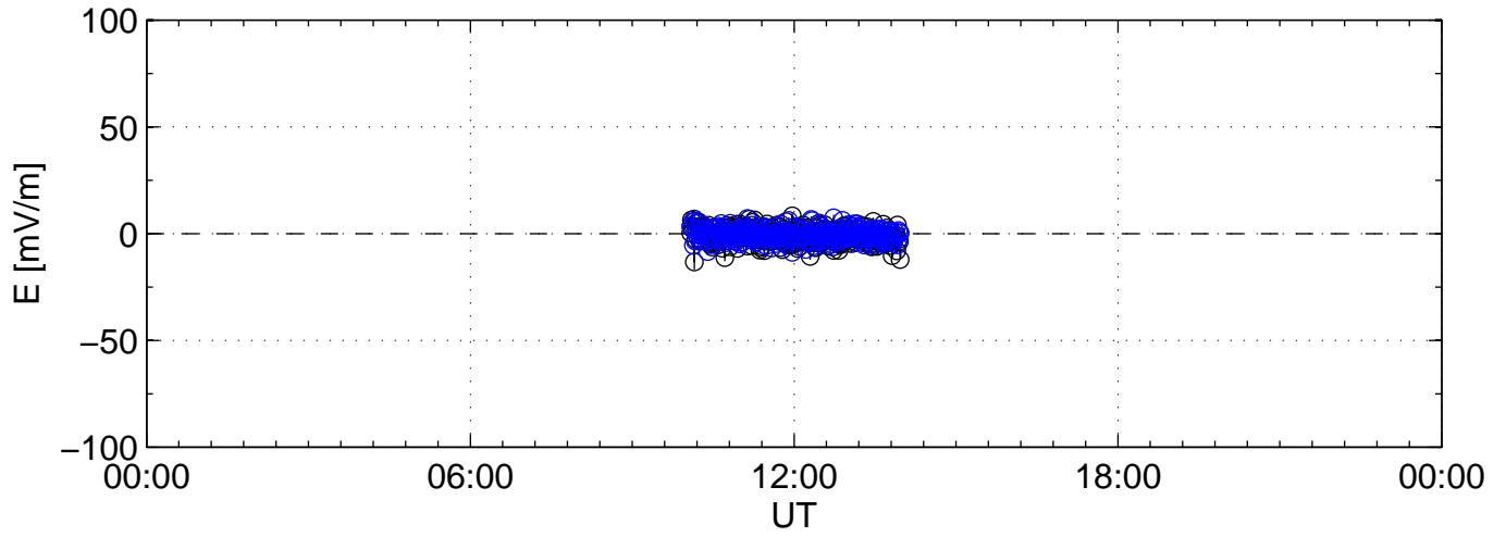
2009-09-17 kst beat 0060sec black:North, blue:East
