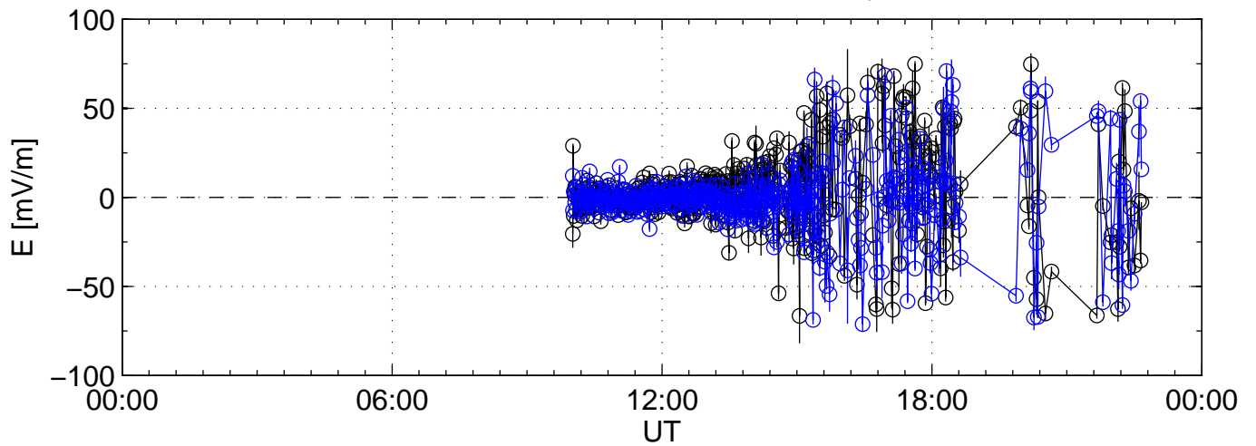
2010-01-18 kst beat 0000sec black:North, blue:East
