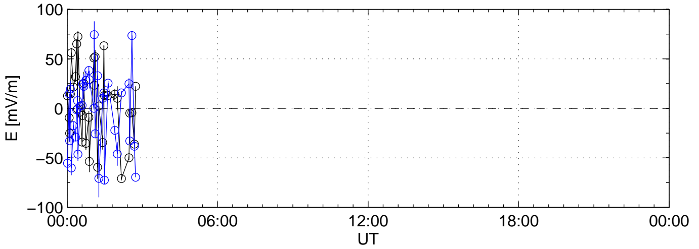
2010-01-19 kst beat 0060sec black:North, blue:East
