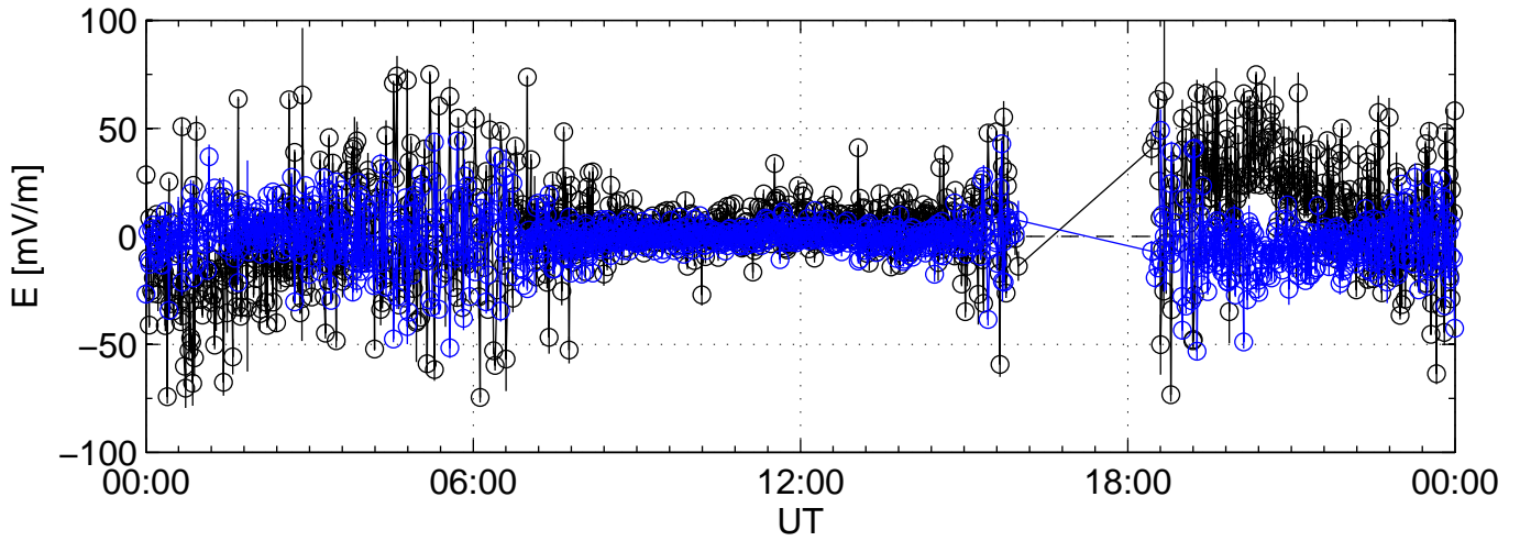
2011-02-02 kst beat 0000sec black:North, blue:East
