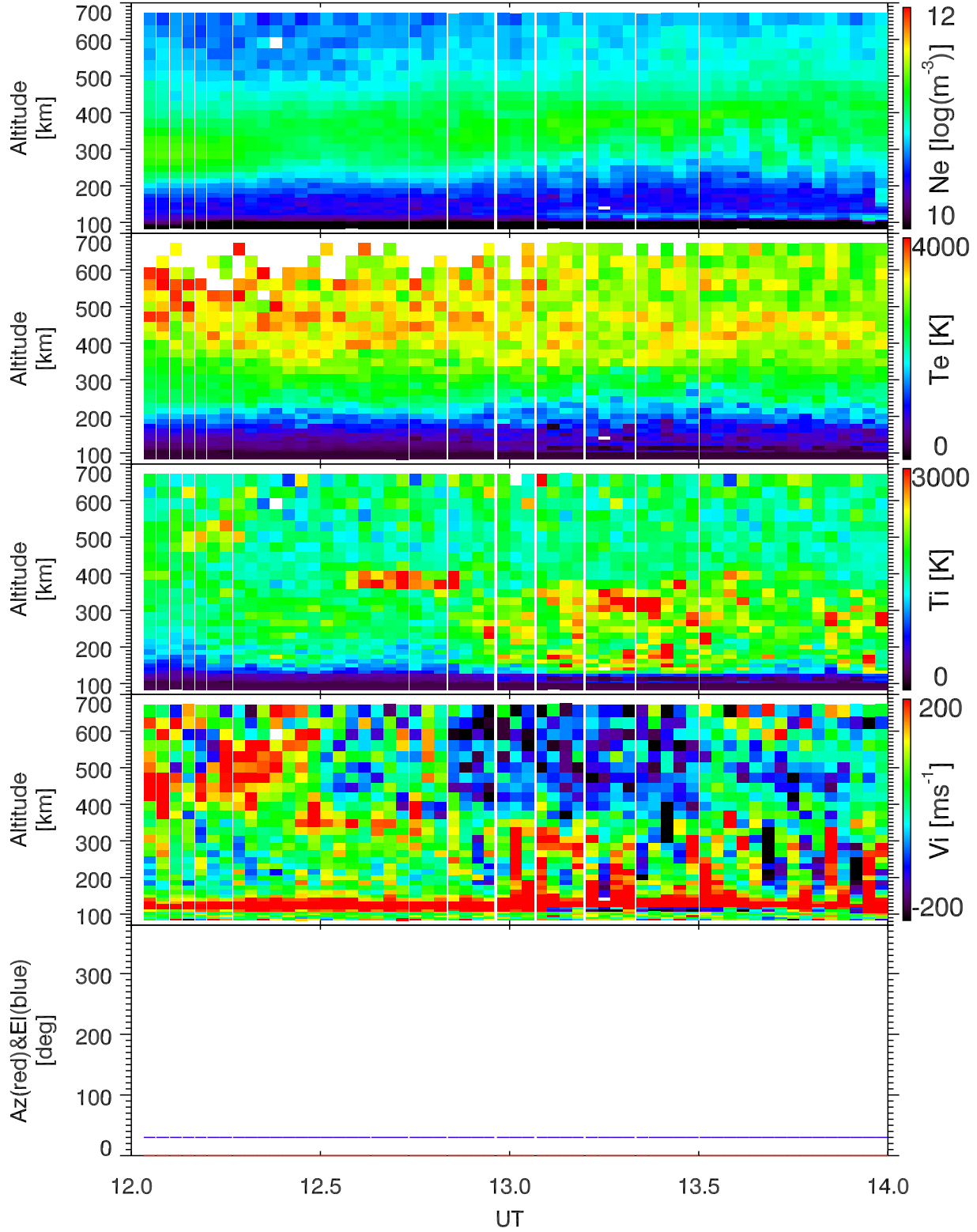
EISCAT 2001-10-10_12_14UT_tau1a_120@vhfa.
