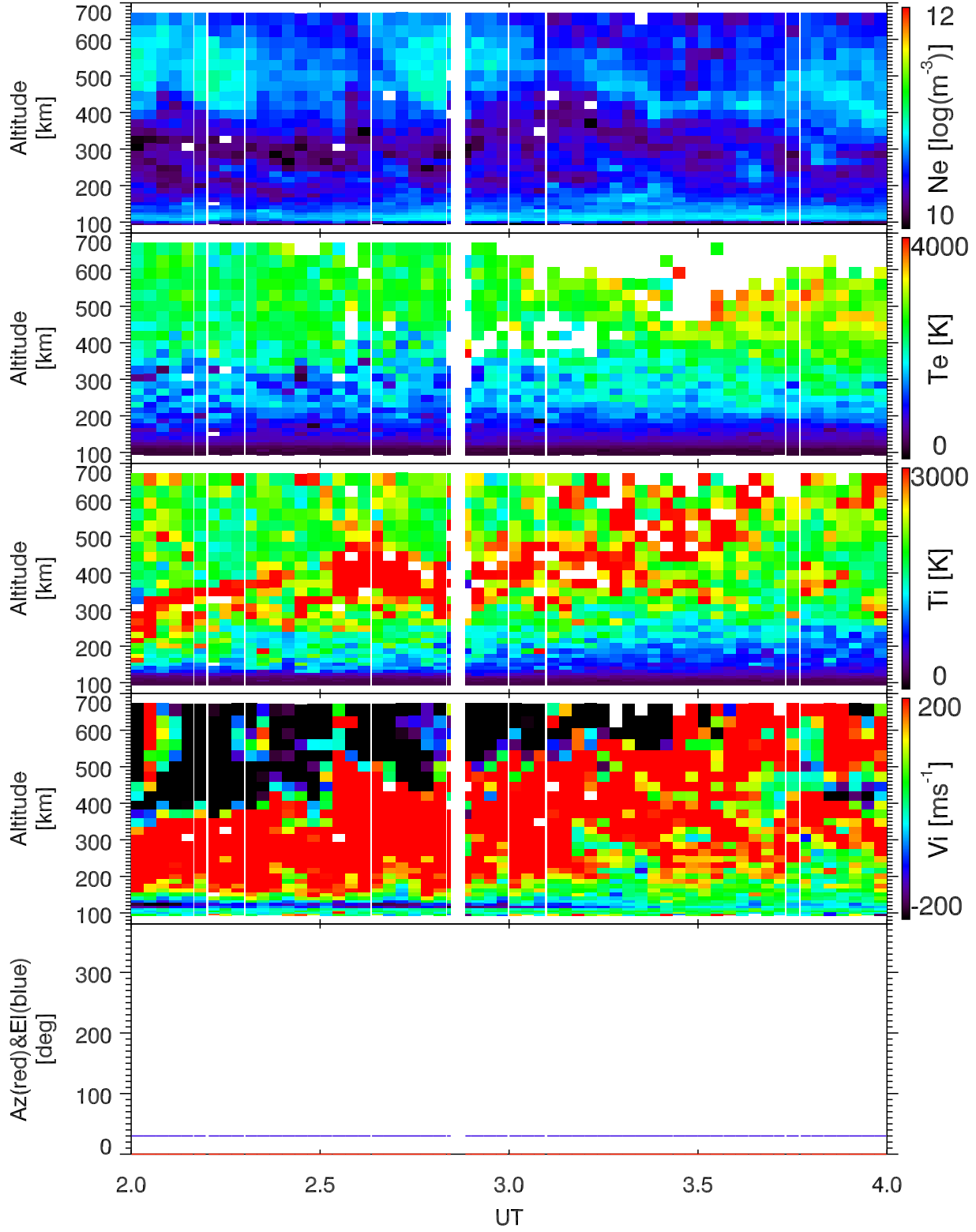
EISCAT 2001-10-11_02_04UT_tau1a_120@vhfa.
