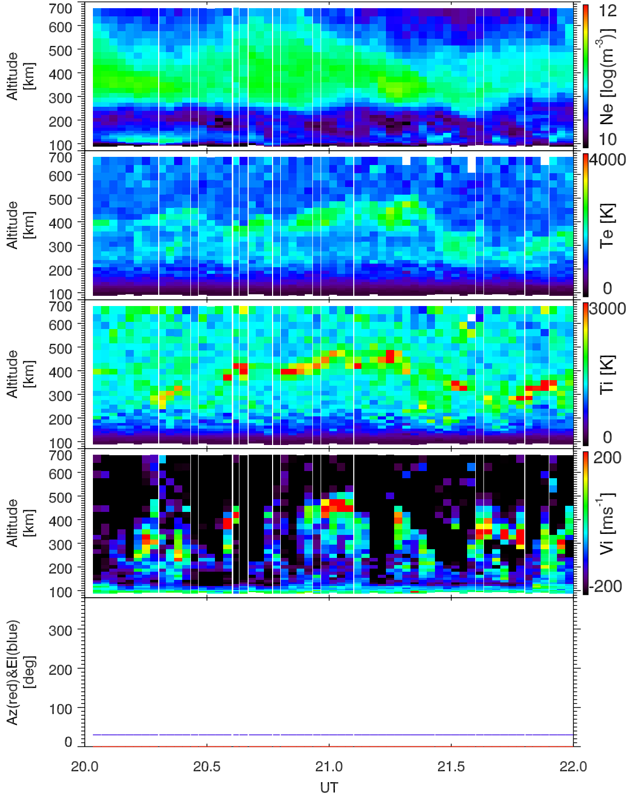
EISCAT 2001-10-13_20_22UT_tau1a_120@vhfa.
