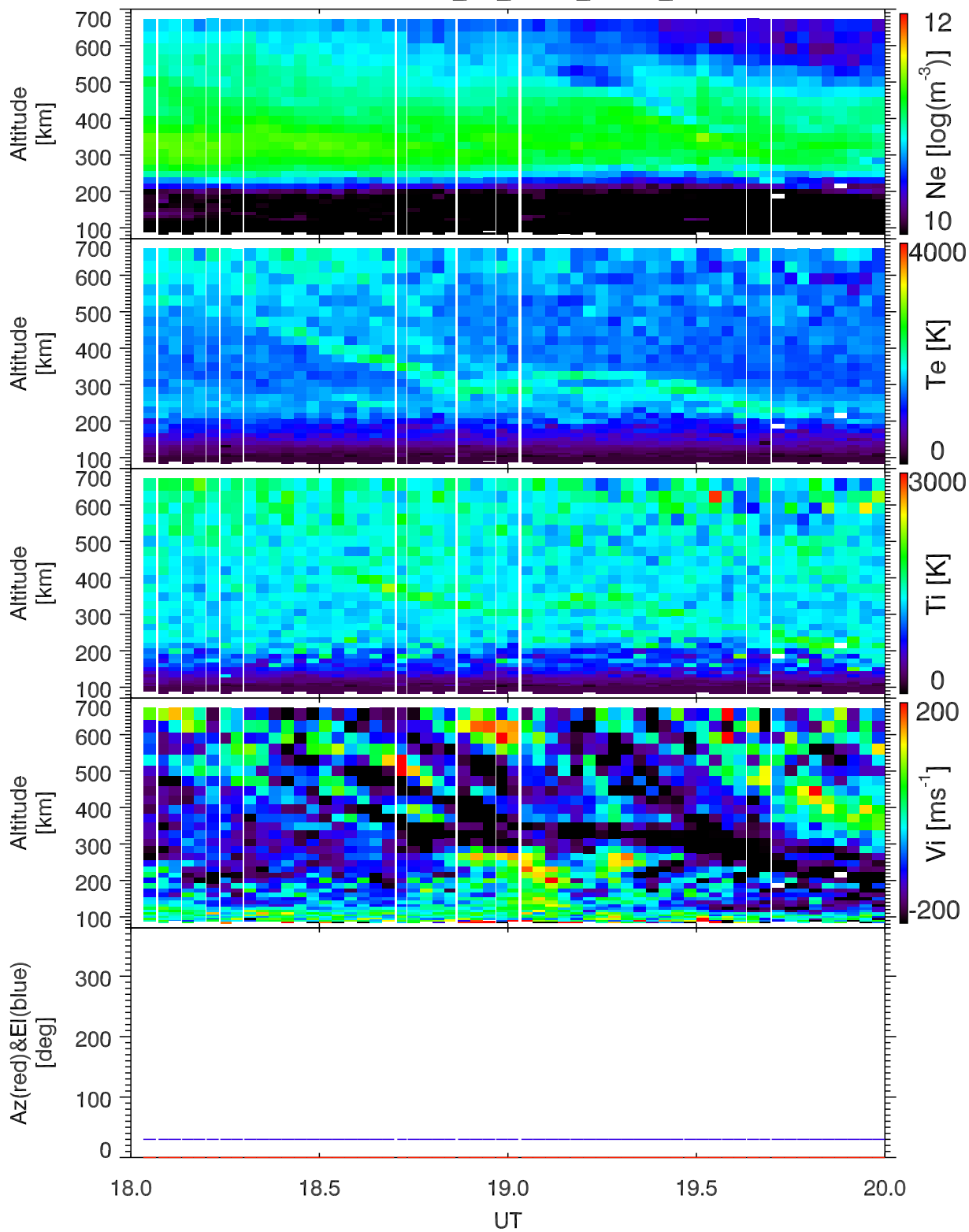
EISCAT 2001-10-15_18_20UT_tau1a_120@vhfa.
