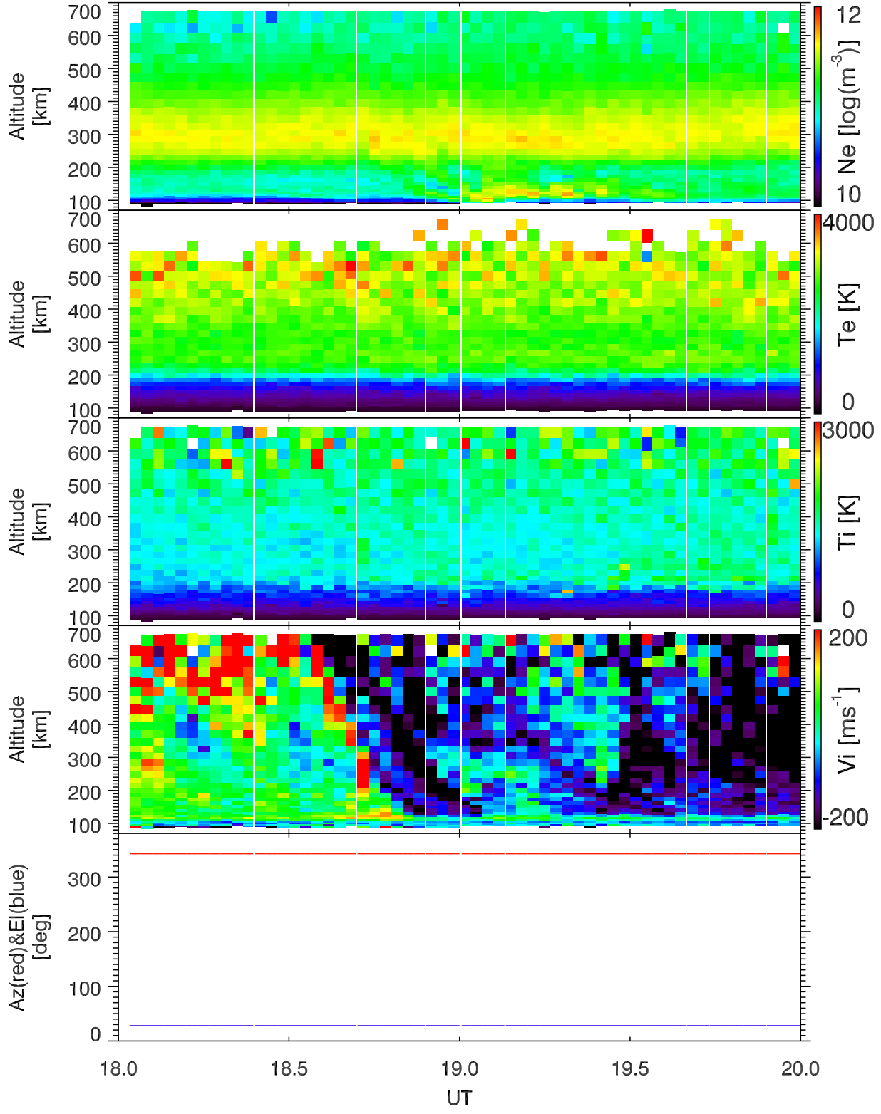
EISCAT 2002-08-13_18_20UT_tau1a_120@vhfb.
